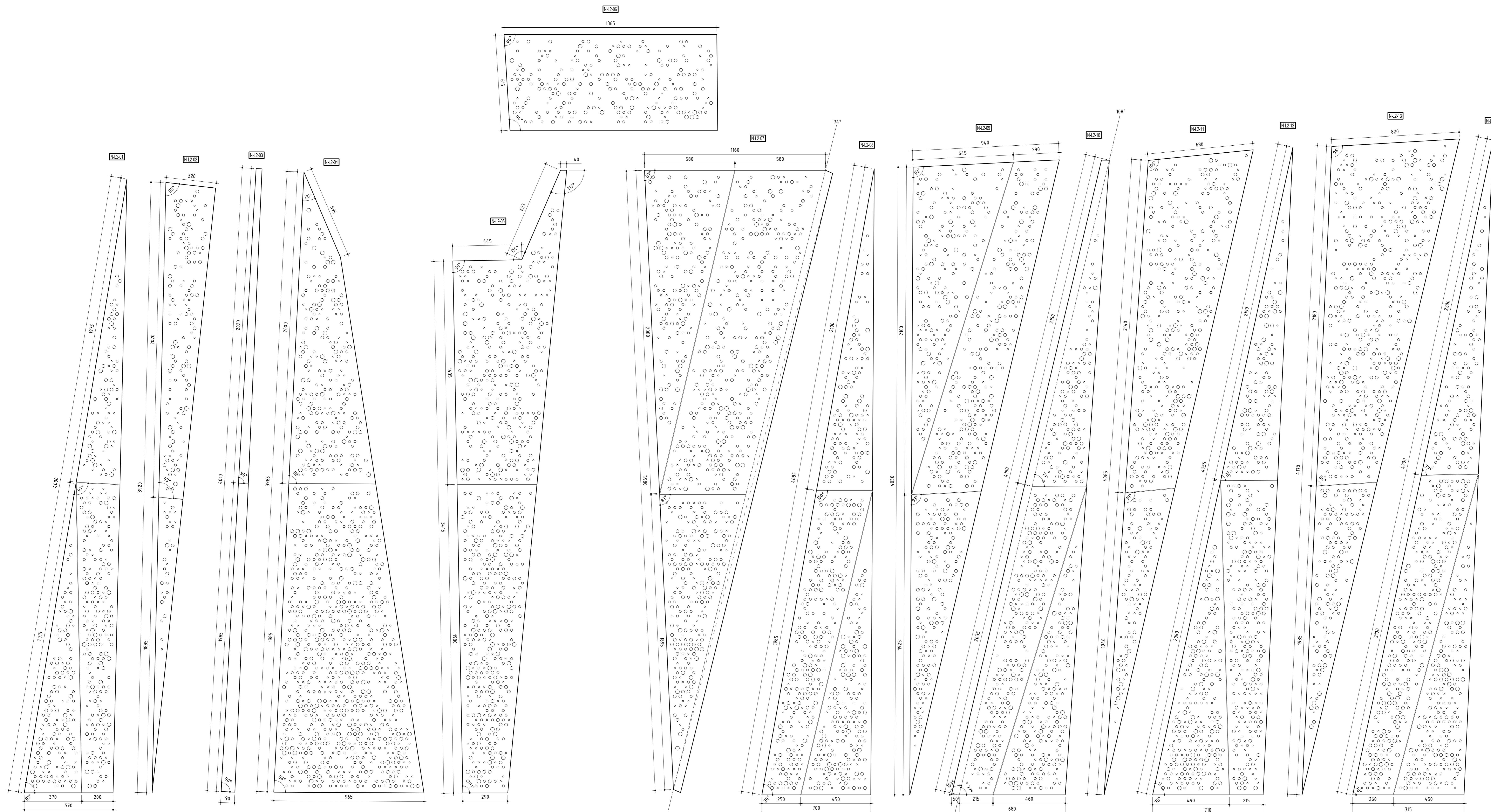
01 UNFOLDED PANELS: N-L2-01 THROUGH N-L2-14 SCALE 1:10
